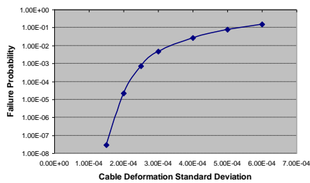
Figure 17. Failure probability in function of cable deformation standard deviation
