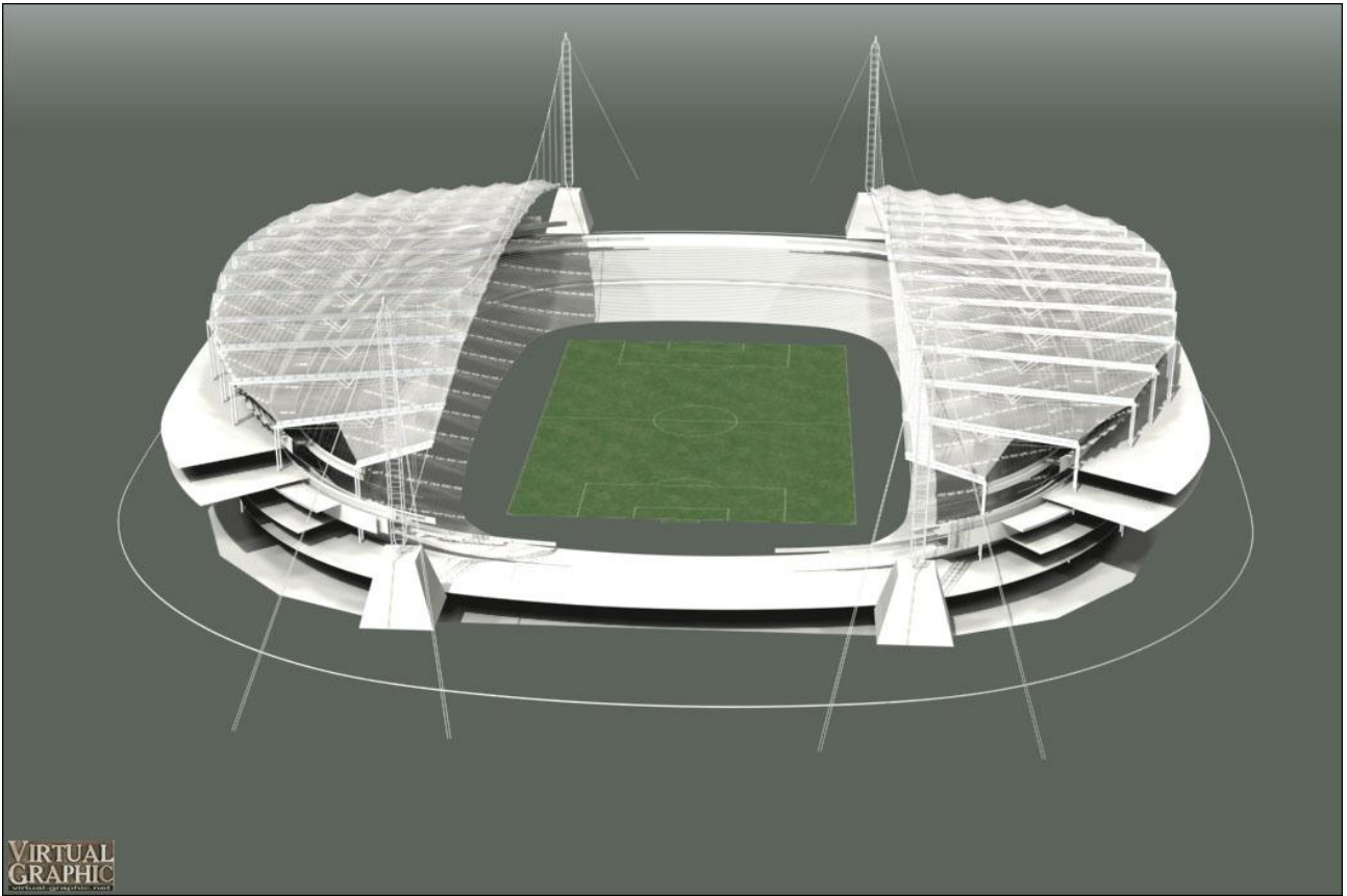
Fig.2 Prestressed tension structure suspended roof
