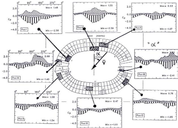
Figure 12 Panel loading as a function of wind direction
