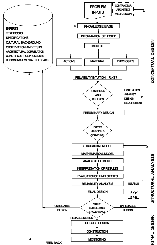
Figure 3 Conceptual design and analysis of structures.
