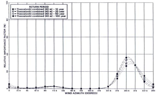
Figure 16 Relative contribution of Azimuthal Direction to the exceedance probability of various return period wind speeds for Thessaloniki, Greece
