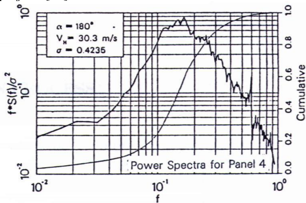
Figure 13 Typical spectra of panel loads
