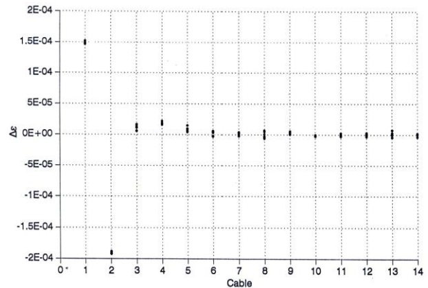
Figure 25 Most Probable \Delta\varepsilon at failure load case 1
