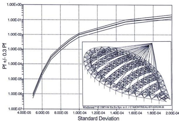
Figure 24 Failure probability for load case 1
