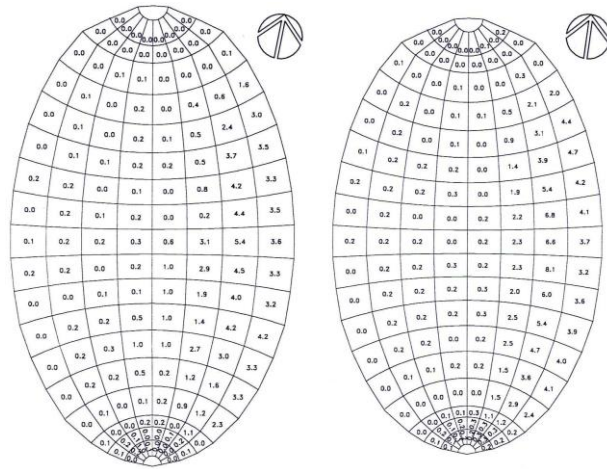
Figure 9 Comparative analysis of snow loading distribution in function of roof shape (10-13m)
