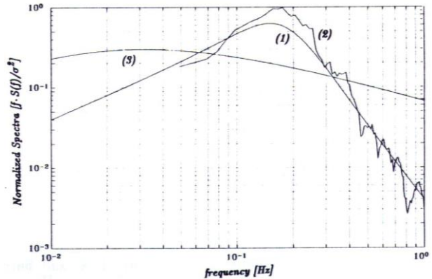
Figure 21 Target (1), simulated (2) and Kaimal's (3) normalized spectra of wind velocity
