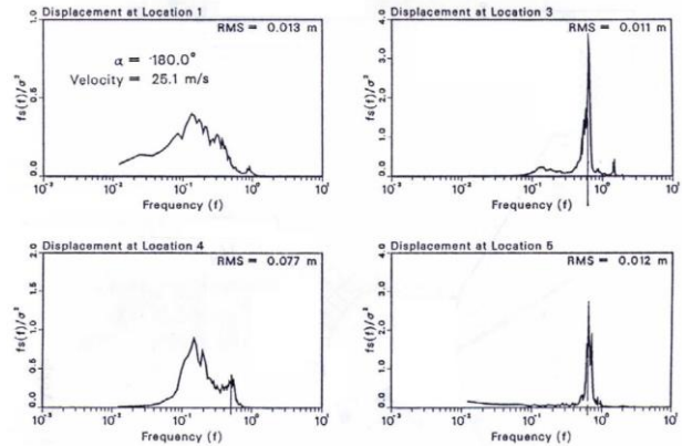
Figure 14 Selected spectra of roof deflections
