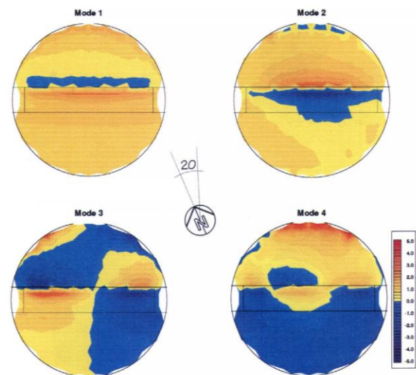
Figure 18 Orthogonal decomposition: pressure mode shapes
