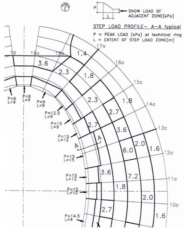
Figure 10 Sliding and wind snow accumulations step loads
