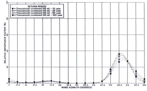
Figure 16 Relative contribution of Azimuthal Direction to the exceedance probability of various return period wind speeds for Thessaloniki, Greece
