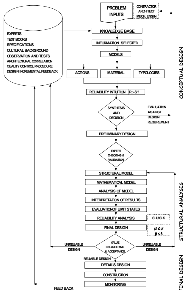
Figure 3 Conceptual design and analysis of structures.
