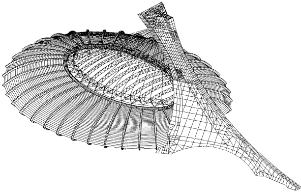
Figure 23 Montreal Stadium cable stayed rigid roof - numerical model
