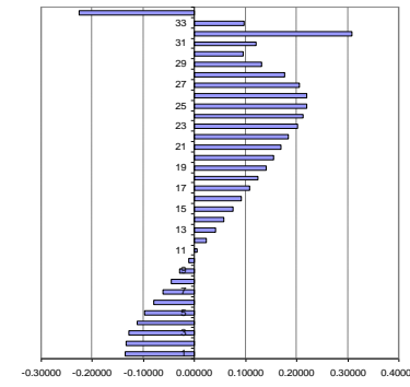
Figure 18. Most probable \Delta\varepsilon in each cable at failure for load comb. 7
