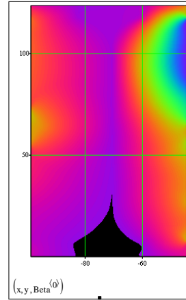
Figure 16. \beta -Safety Index distribution, evidencing SLU sensibility on black region ( \beta=3.798 )
