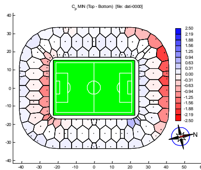
Figure 8. Maximum and minimum values of net pressure coefficients (wind direction: 0°).
